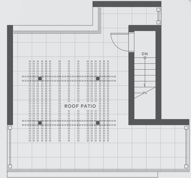
UPPER FLOOR
